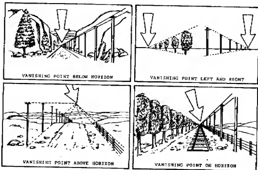
Figure 4-18. Vanishing points.
